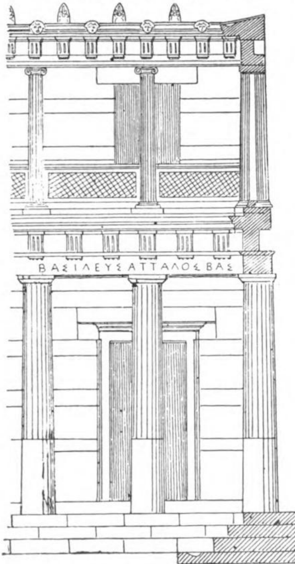
porticus regis Attali, Athenis in foro exstructa
